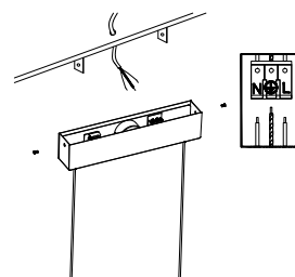
Connect the wires
