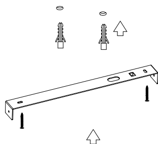
Drill holes & apply plastic anchors With screws
