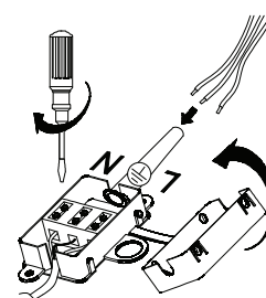
Connect the wires
