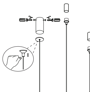
Apply side screws and make Hanging elements stable
