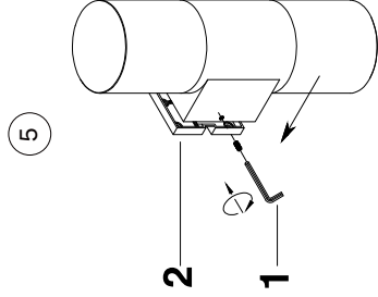
Put in place & apply screws
