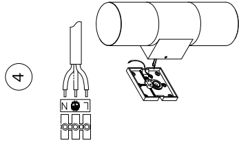
Connect wires
