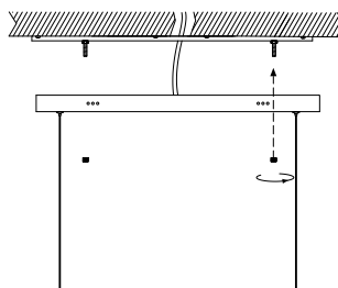
Apply the bottom screws
