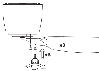
9. Attach the wings by applying the screws
