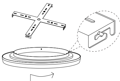
8. Fix the product in to place
