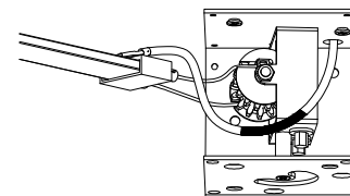
9. Connect the wires
