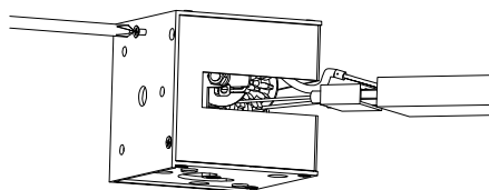
11. Install the decorative cover
