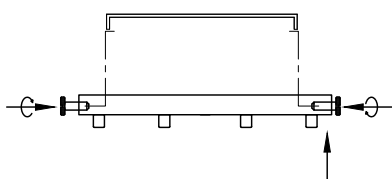
4 Apply the side screws
