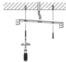
4 Apply screws
