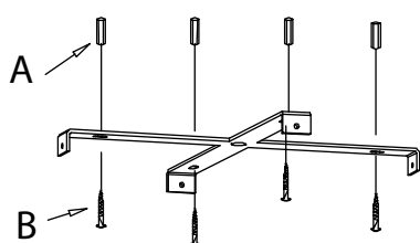
3. Apply plastic anchors with screws
