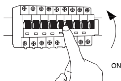
9. Turn on the general switch
