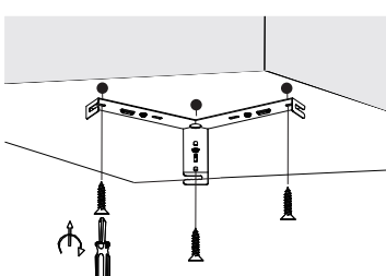
5. Apply screws
