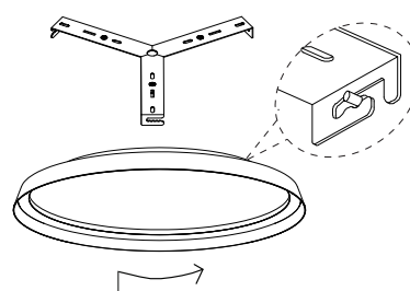
8. Apply the product by rotating
