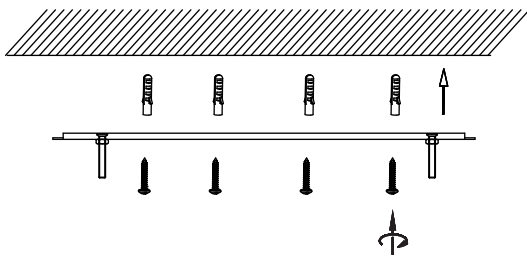
Align, mark & drill hole, apply plastic anchors & tie up the screws
