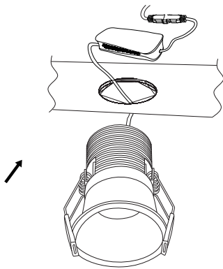
3. Connect wires
