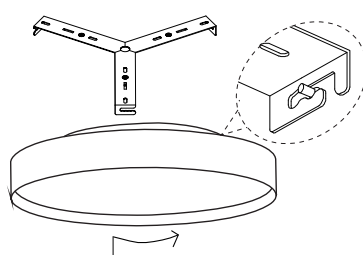
8. Put the product in place
