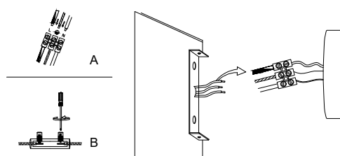
4. Connect the wires
