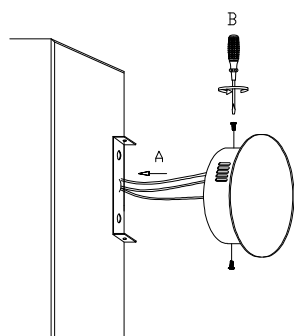
5. Apply the side screws
