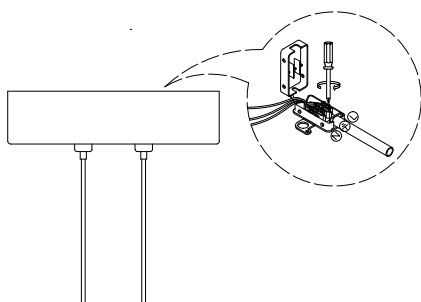
3. Connect wires
