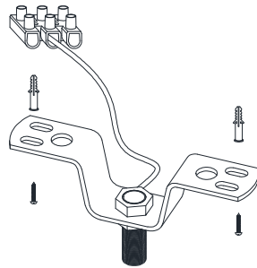
Apply plastic anchors and tie up screws
