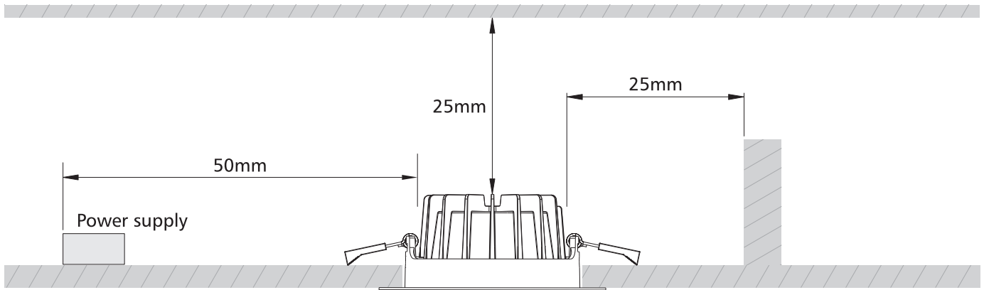
Fig 1: Installation Spacing
