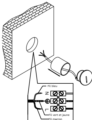
Connect wires
