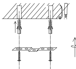
2 Drill Holes, Apply Plastic Anchors & Screws
