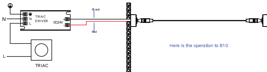
Connect two copper wires to the DC port of the power supply
