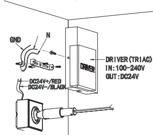
Connect wires for driver and track
