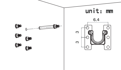
Apply the screws, mark & drill a hole
