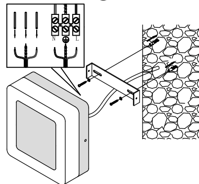
Connect wires
