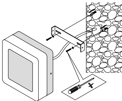
Mark, drill holes, apply plastic anchors with screws
