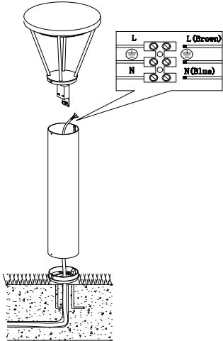
4. Connect wires
