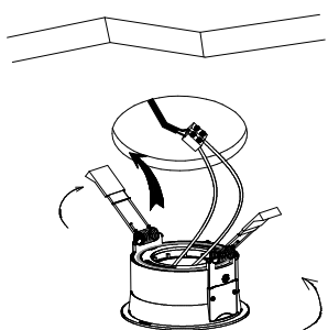
3. Apply the product and make it stable
