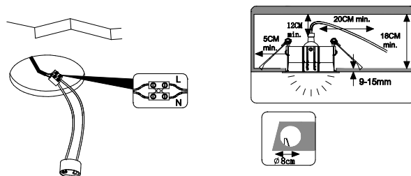
2. Connect the wires
