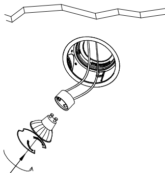
4. Place the bulb in place
