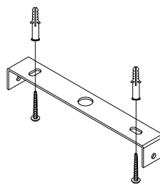
2 Align, mark and drill holes
