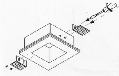
Apply the side screws
