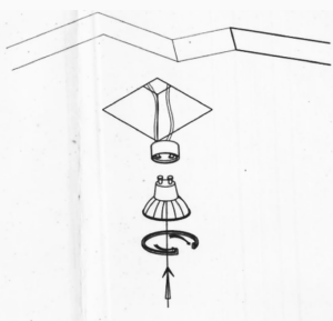
Apply the bulb by rotating
