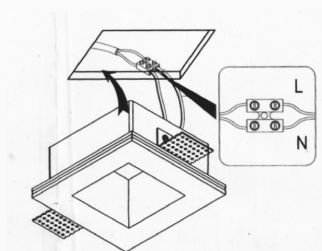
Connect the wires
