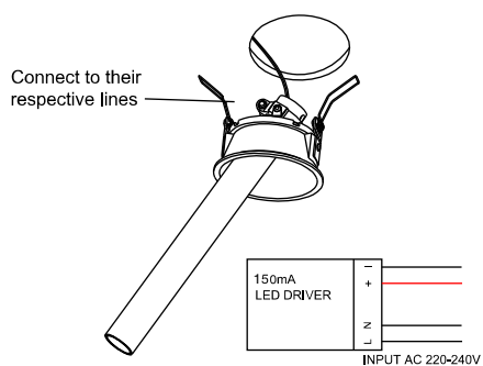
Connect the wires of the driver
