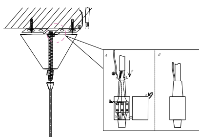
3 Connect The Wires
