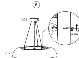
Apply screws
