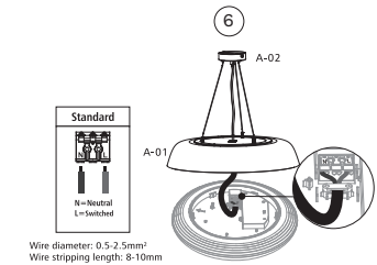
Connect wires
