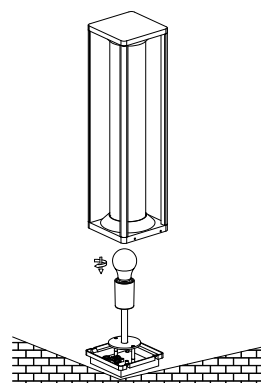
4. Insert bulb & apply the lid
