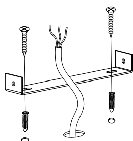
3. Align, mark and drill holes To apply the screws
