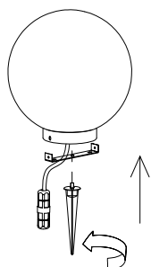
3. Align, mark and drill holes To apply the screws
