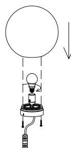
2. By rotating, break it apart
