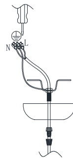
Connect wires
