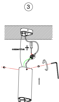
Connect the wires & put it in place by applying the side screws
