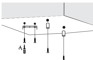
Apply screws
