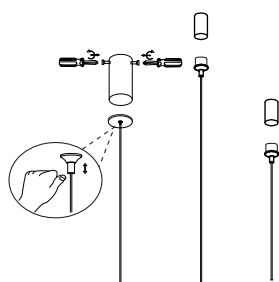
Apply side screws and make hanging elements stable
