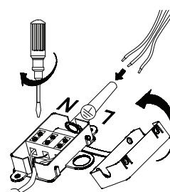
Connect the wires
