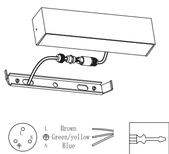
Connect wires
