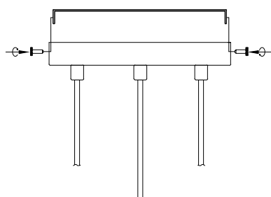
Apply the side screws
