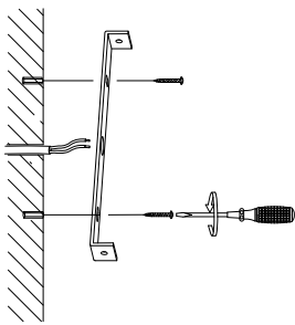
Tie up the screws To make it stable
