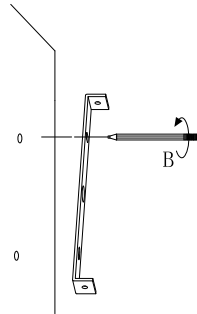
Mark where to drill holes
