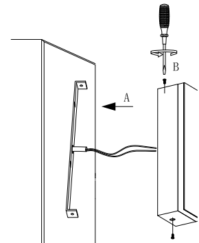
Apply side screws
