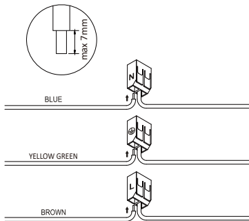
5. Connect the 3 wires
