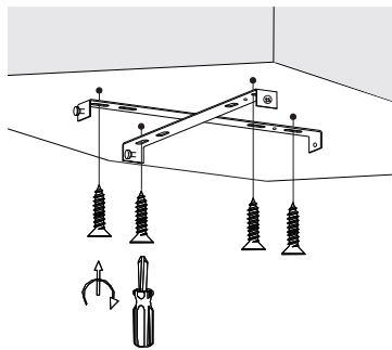
5. Apply screws
