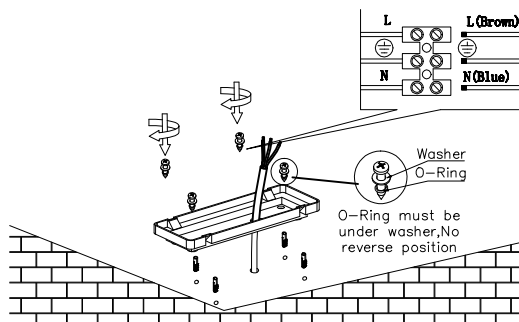
Fix the base on the ground by applying anchors with screws & connect wires
