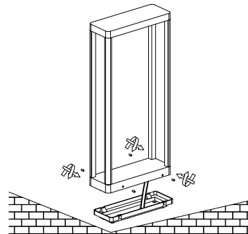
Install cable & tie up screws to make it stable
