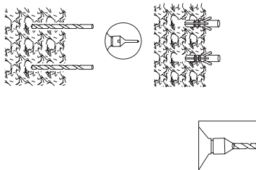
Drill holes & apply anchors
