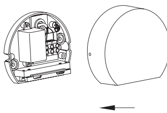
Apply the cap into place
